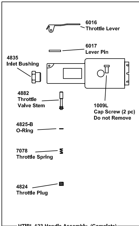
HTIBL 123 Handle Assembly, (Complete)
