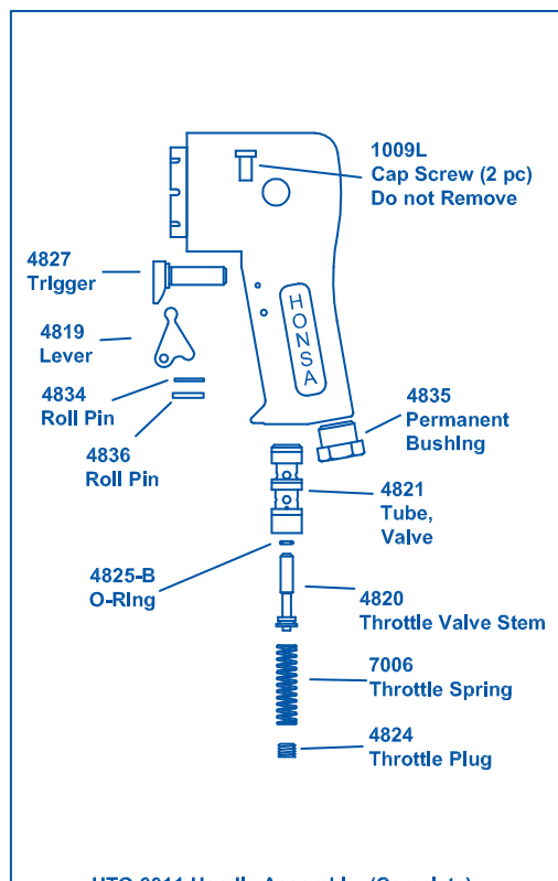
HTO 6011 Handle Assembly, (Complete) HTO 6011S Handle Assembly for "WT" Series, (Complete)
