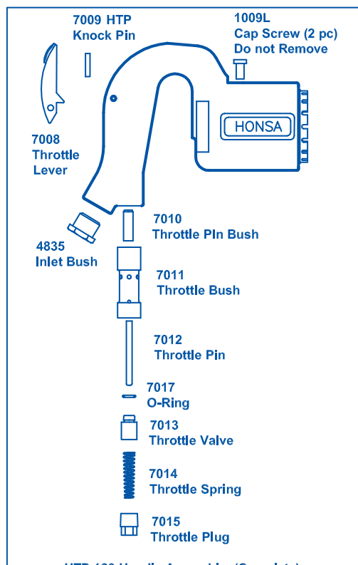
HTP 123 Handle Assembly, (Complete) HTIBL 123S Handle Assembly for "WT" Series, (Complete)
