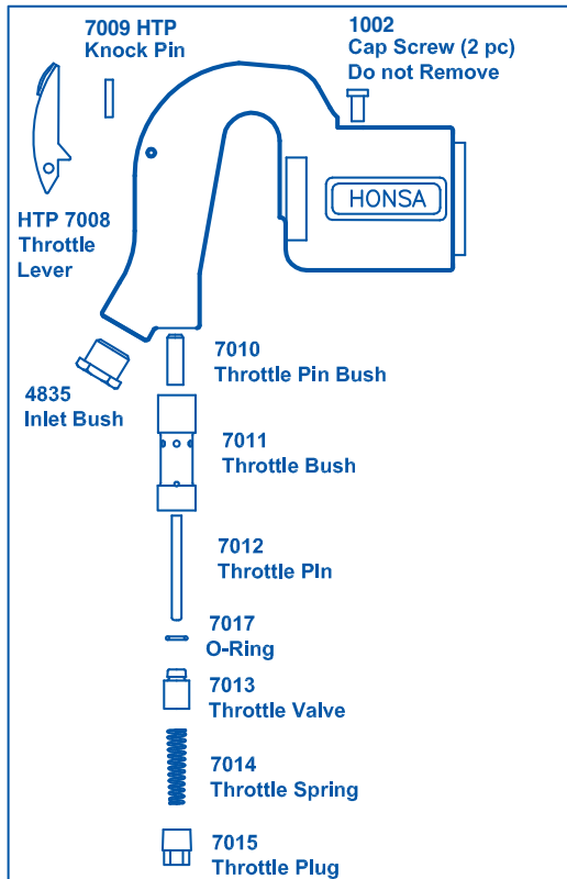
B2500 Handle Assembly, (Complete)
