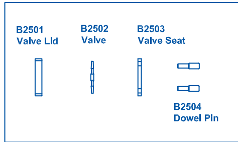
B2575 Valve Assembly, (Complete)
