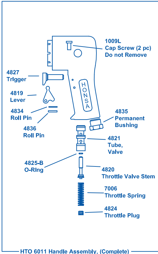
HTO 6011 Handle Assembly, (Complete)
